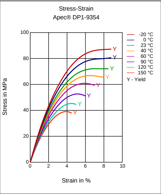
Stress-strain
